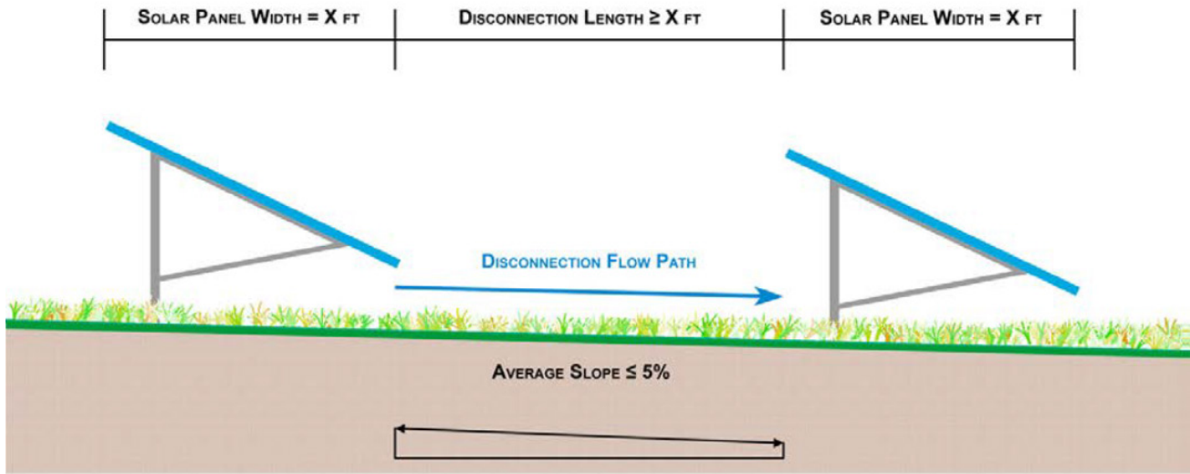
Figure 13-2: Typical Solar Panel Installation with Slopes > 5\% and \leq 10\%
