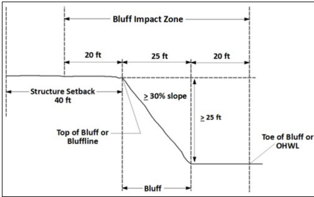
Figure 11-2: Natural Escarpment Bluff and Bluff Impact Zone
